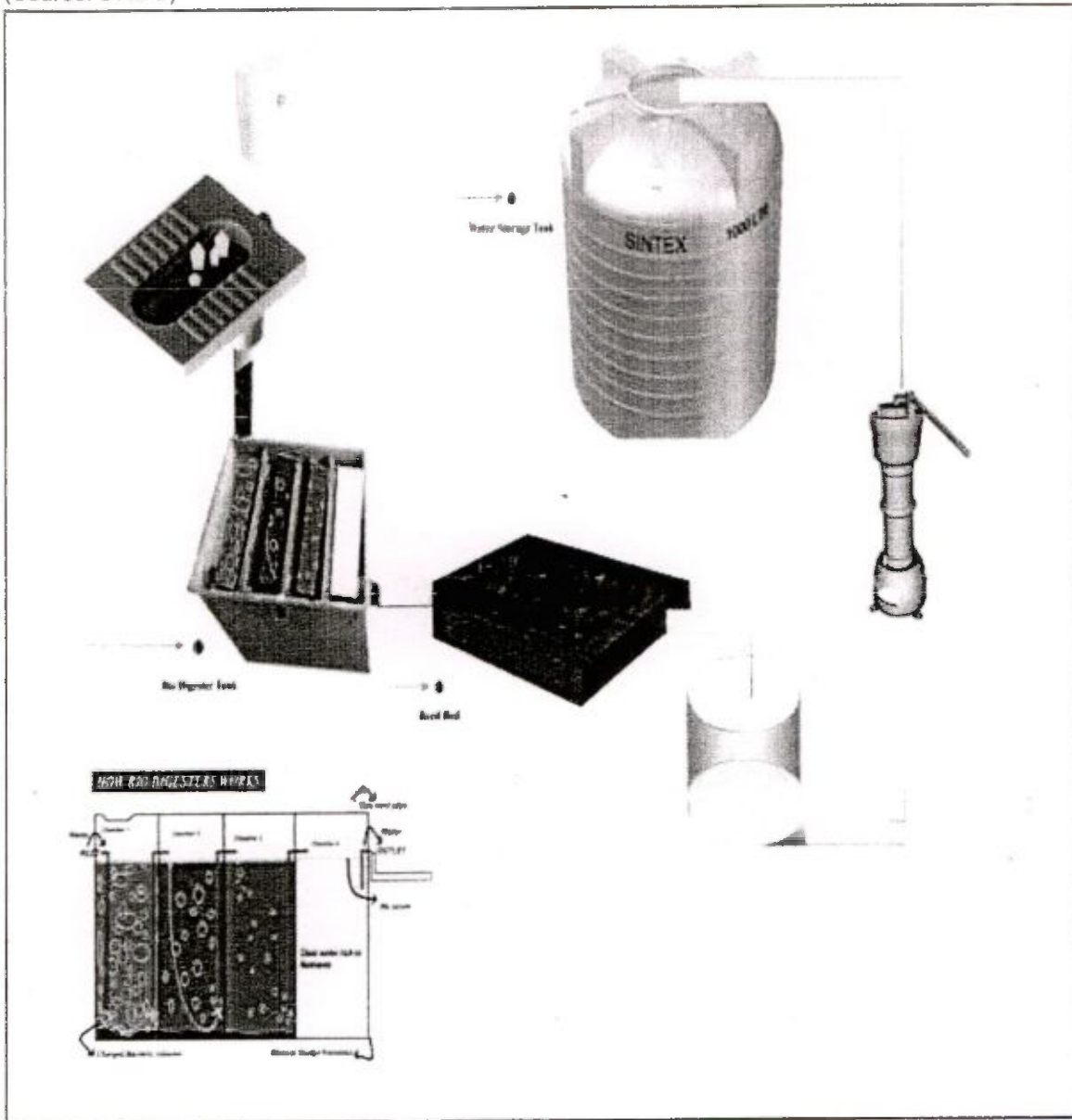
Figure 7: Details of bio-digester with reed bed
