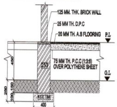
125 MM THK. BRICK WALL
