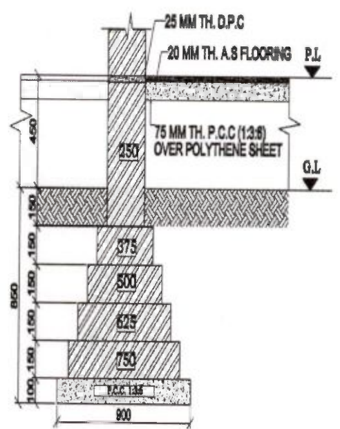
250 MM THK. BRICK WALL
