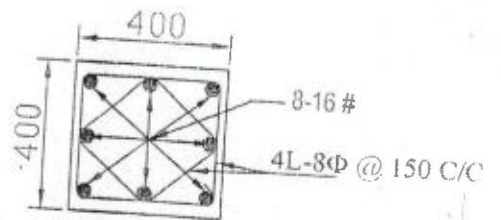
SEC. AT P-P FOR COL. (400x400)
