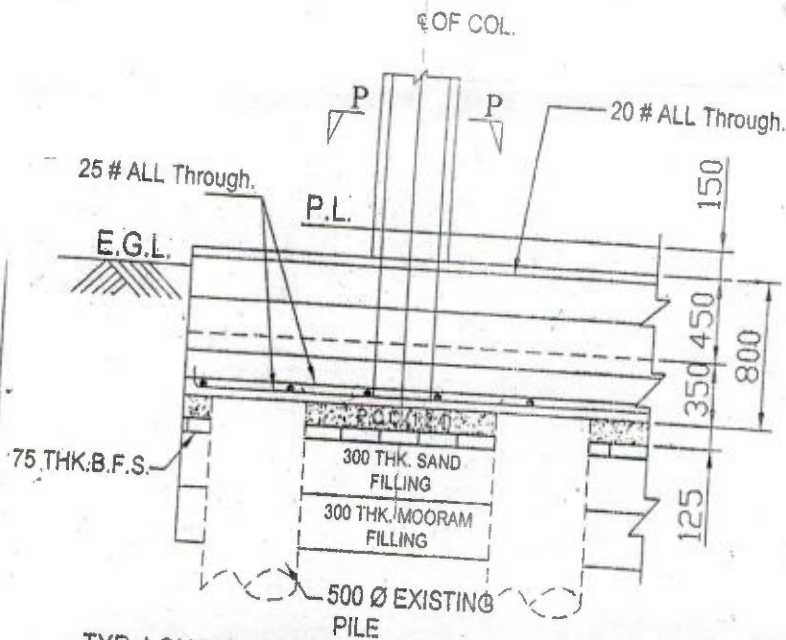
TYP. LONG SEC. OF R.C.C. RAFT BEAM FOUNDATION
