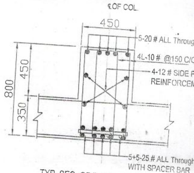
TYP. SEC. OF R.C.C. RAFT BEAM MARK-RIB
