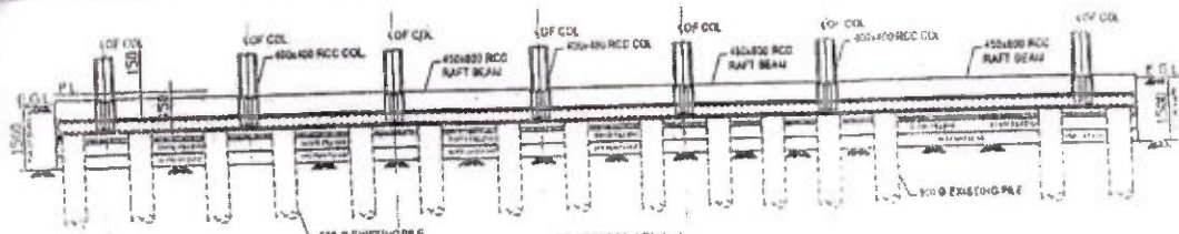
SECTION AT A-A TYP. SECTION OF RAFT FOUNDATION
