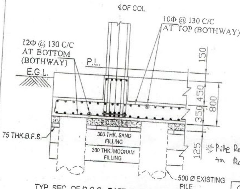
TYP. SEC. OF R.C.C. RAFT SLAB FOUNDATION
