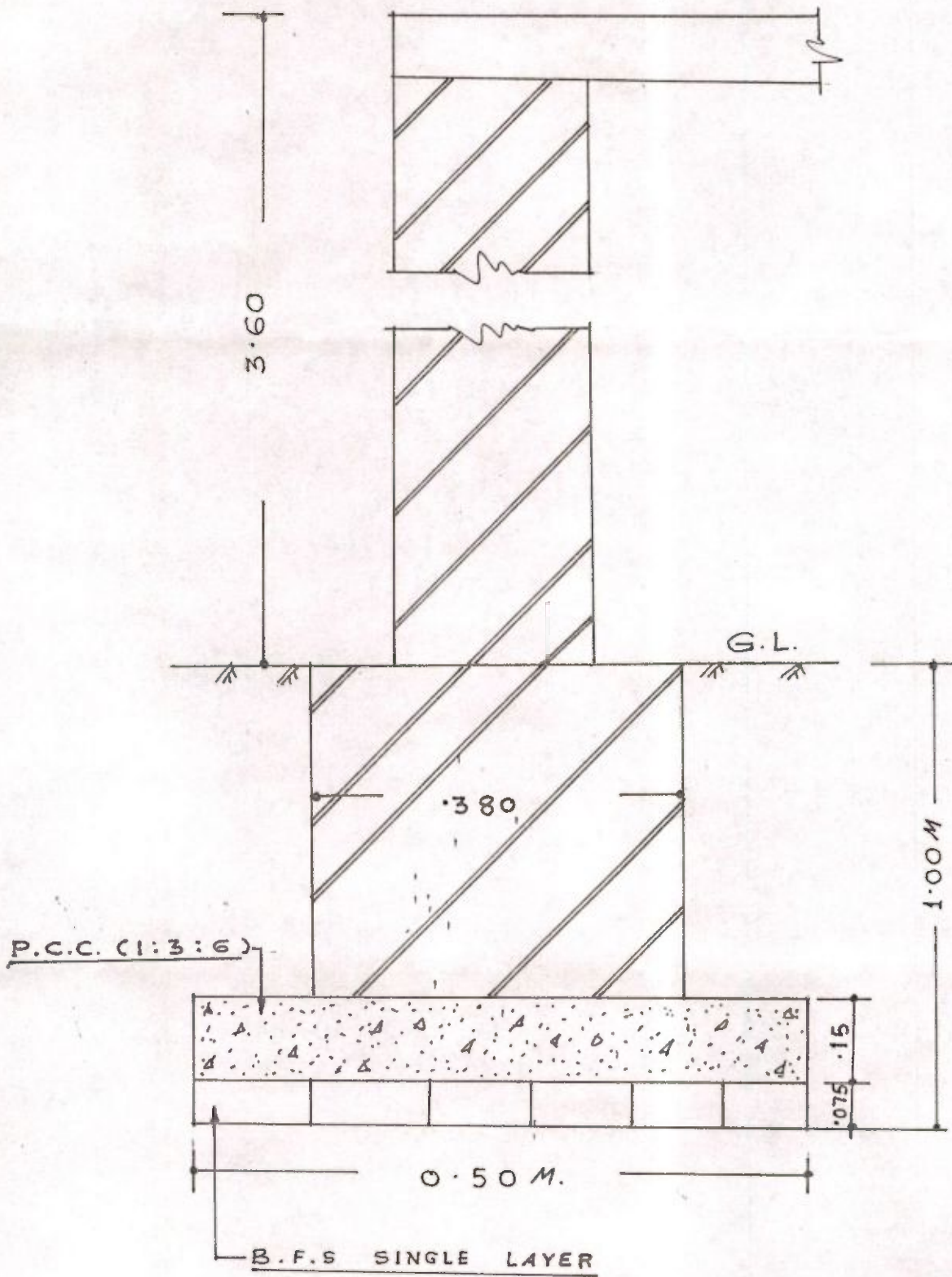
TYPICAL BRICK WALL FOUNDATION
