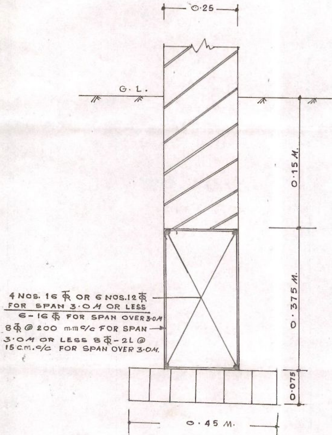
TYPICAL PLINTH BEAM FOUNDATION
