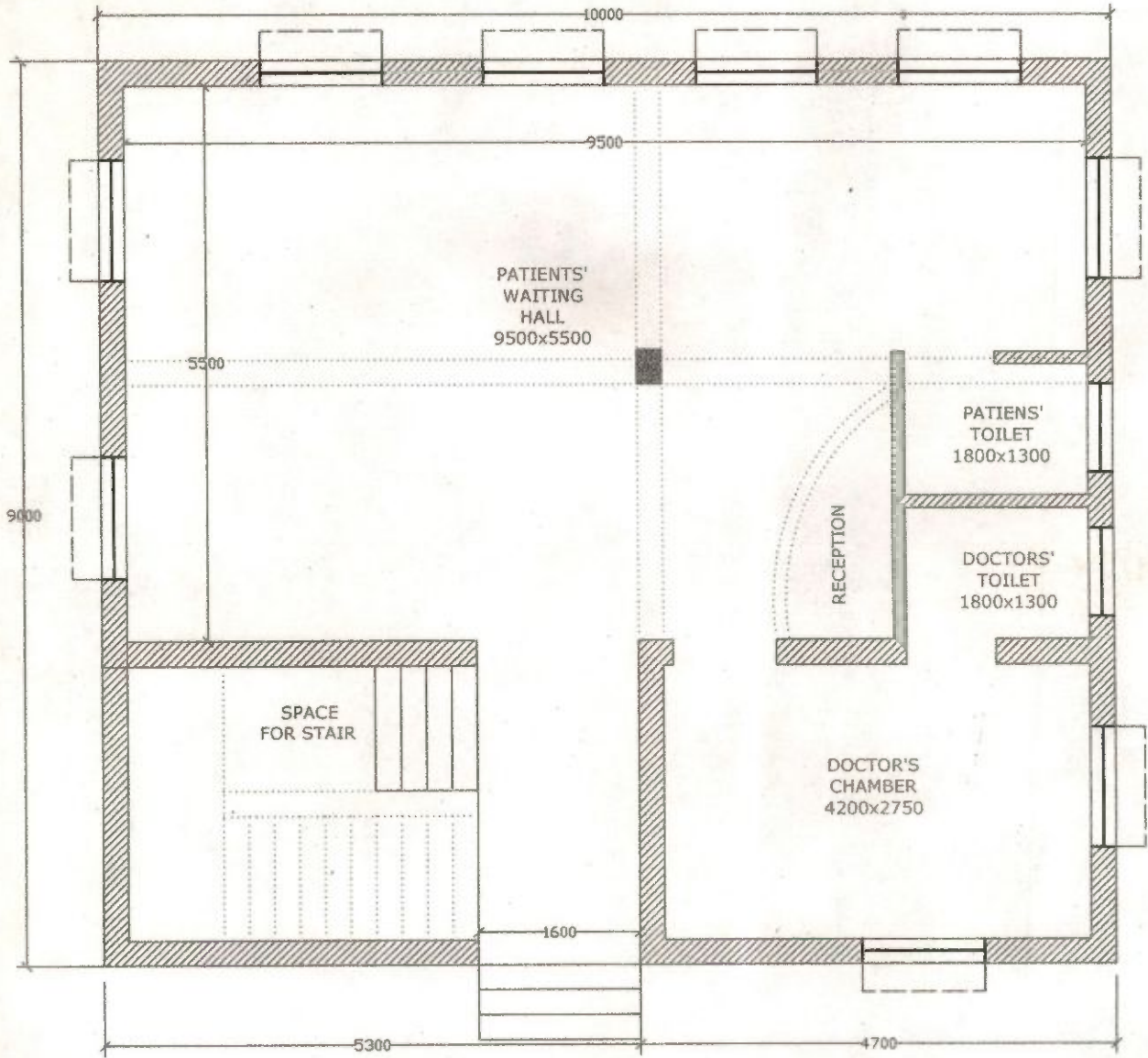
TYPICAL DRAWING HEALTH SUB CENTRE PLINTH AREA 90 sqM
