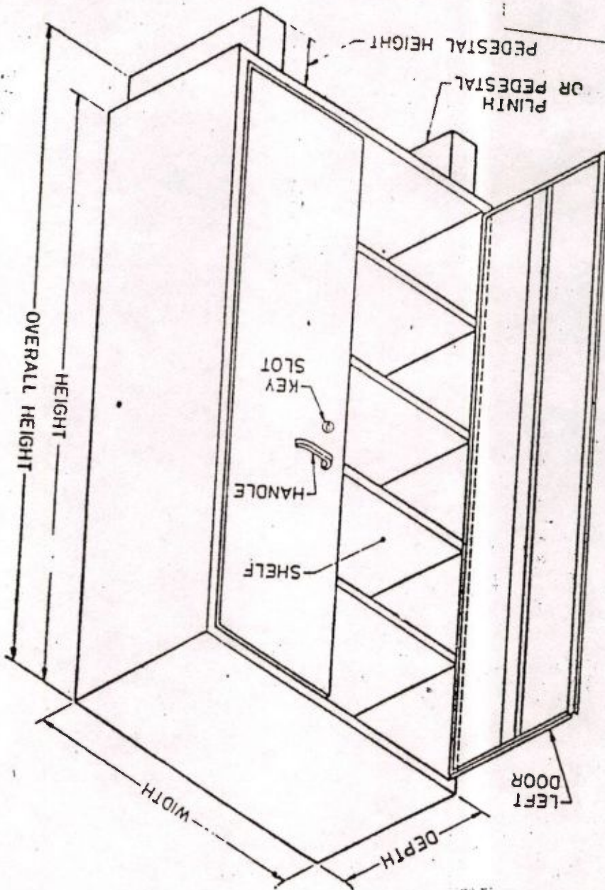
TYPICAL SKETCH OF STEEL ALMIRAH
